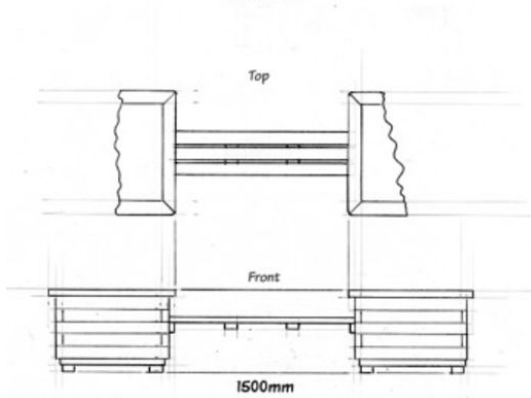
WOODEN SEAT LINKING TWO 1000MM PLANTERS 1500mm
